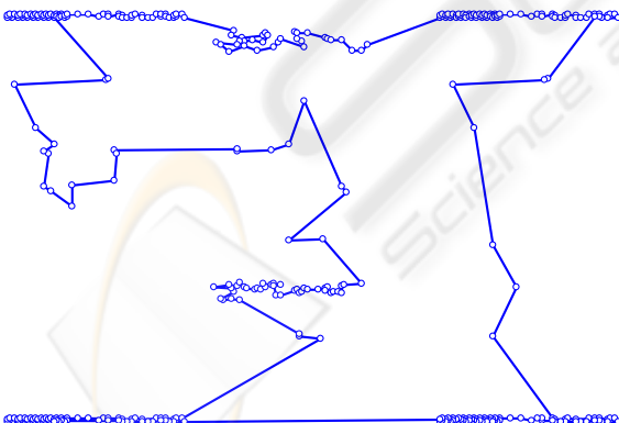
Figure 5: Example of the fl417 problem with the application of Wang's Neural Network with the soft WTA principle and 2-opt, with an average error of 1.43%.
