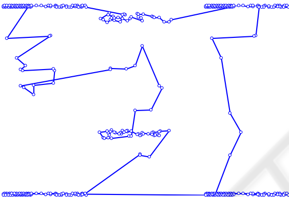
Figure 4: Example of the fl417 problem with the application of Wang's Neural Network with the soft WTA principle and average error of 9.05%.
